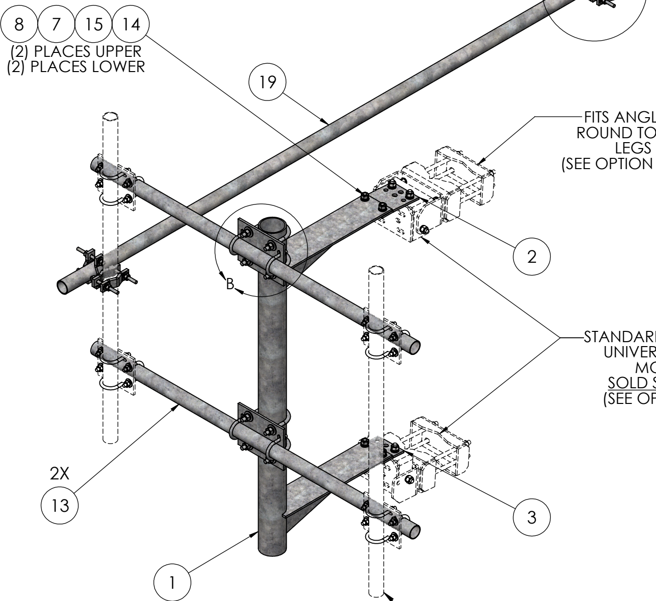
DETAIL B SCALE 1 : 6
